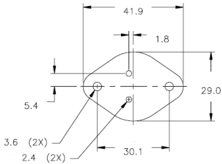
TO-3-05
