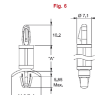
LCBS-6 Top Hole: Snap-lock: \varnothing 4 Panel Thickness: 3.2 Fig. 6
