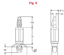
LCBS-8 Top Hole: Snap-lock: 4 \pm 0.08 Panel Thickness: 1.57 Fig. 8
