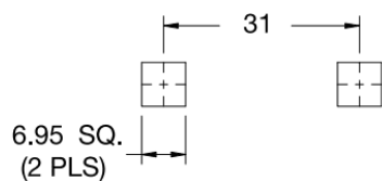
MOUNTING HOLES
