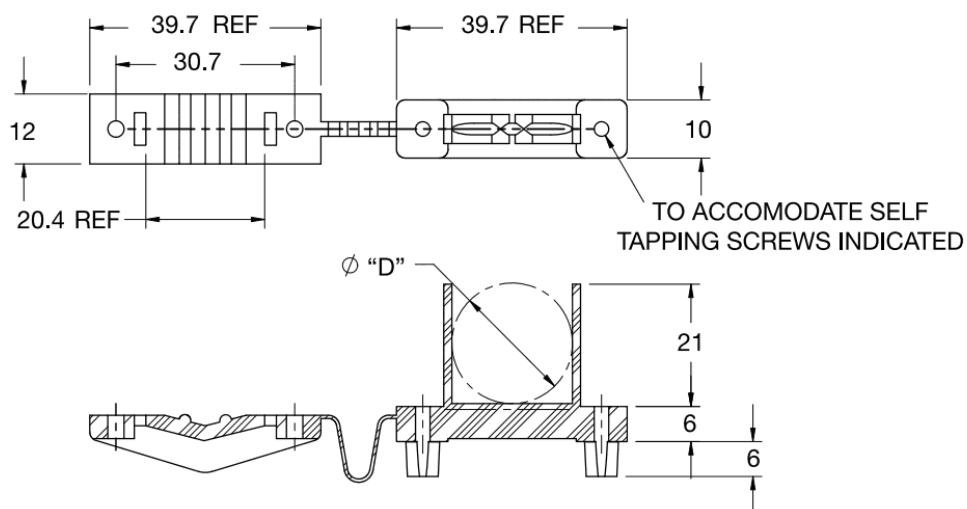
MOUNTING HOLES
