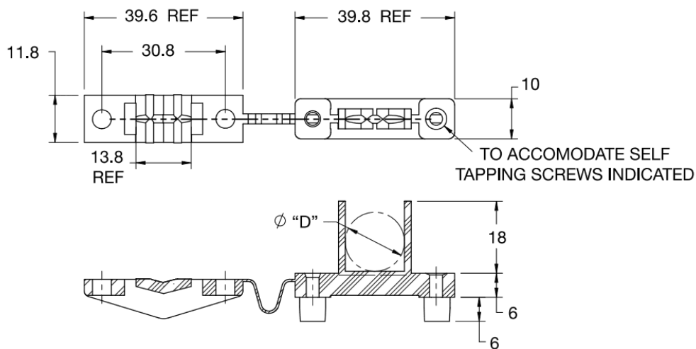
MOUNTING HOLES
