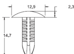
BPF-F3T31
