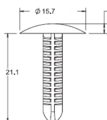
BPF-F3T31
