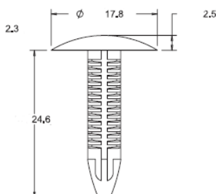
BPF-F1G12
