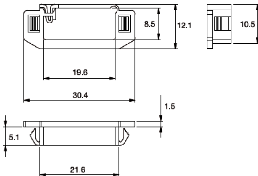
PANEL MOUNTING DETAILS
