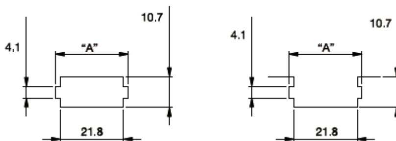
PANEL MOUNTING DETAILS
