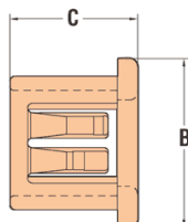
Typ 2 - wiele paneli Type 2 - multiple panel design
