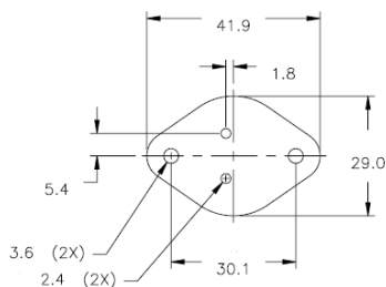
TO-3-05
