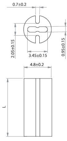
LEDM-2 For T-1 Series LED
