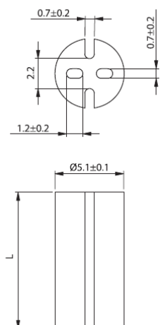
LEDM-1 For T-1 3/4 Series LED
