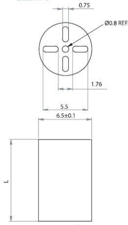
LEDM-3 For T-1 3/4 Series LED
