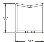
OPTIONAL ADHESIVE BASE 1mm THICK
