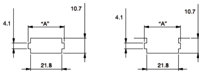
PANEL MOUNTING DETAILS
