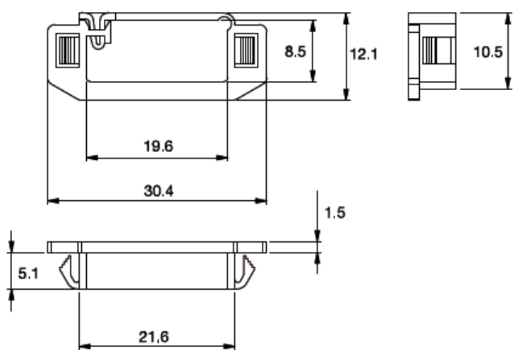
PANEL MOUNTING DETAILS
